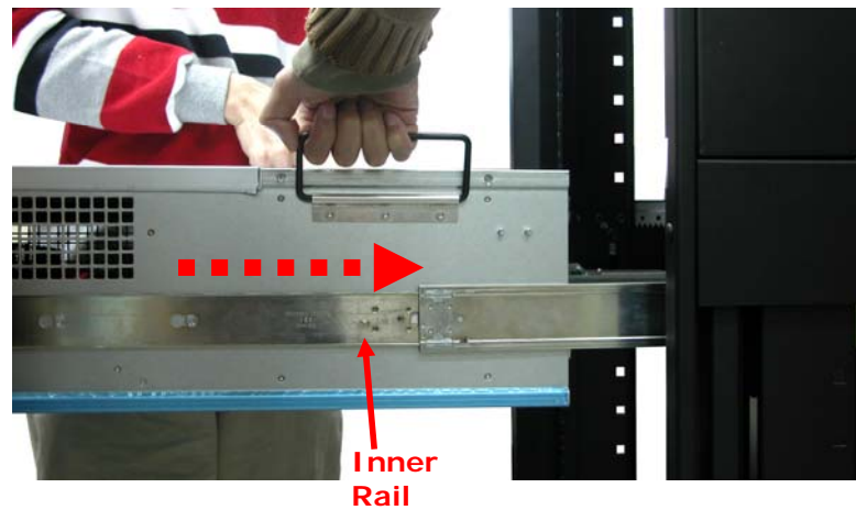
Inner Rail Aligned with and Inserted into the Middle Rail
