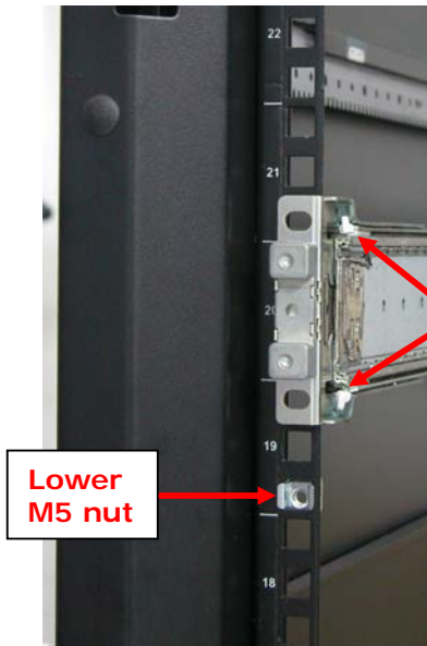
View from Front Side of Front Left Rack Post Lock Lever is Not Locked
